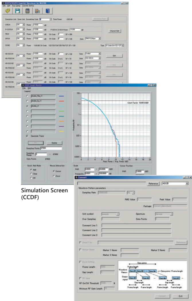
Convert Screen
